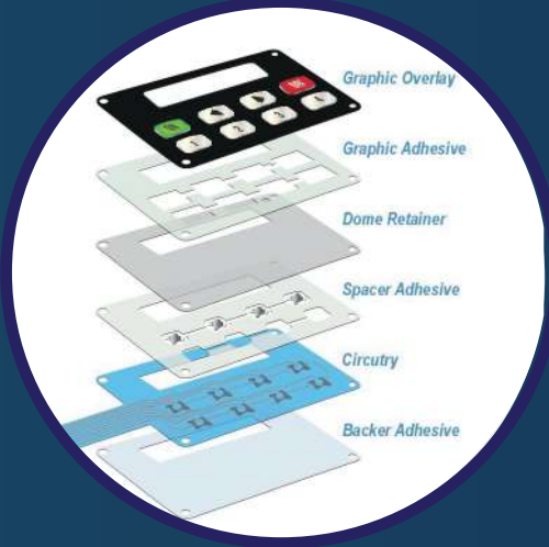
Membrane Switch Panel
